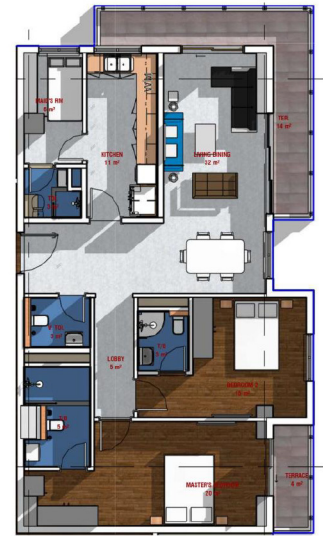
2 BEDROOM APARTMENT (NET AREA = 131 SQM)
